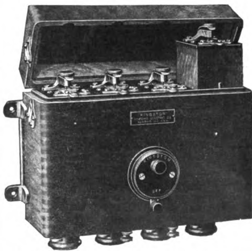
Kingston 4-cylinder Unit System Dash Coll. The most popular coll on the market today
